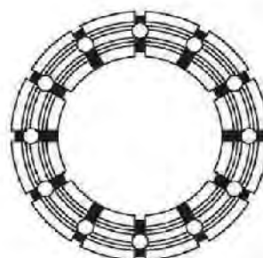
Face Discharge 6mm hole Tapered Waterway (FD6HTWW)
