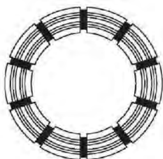
Internal Flush Standard Waterway (IFSWW)
