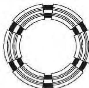
Face Discharge Elongated Holes 9mm Tapered Waterway (FD E/H TWW)
